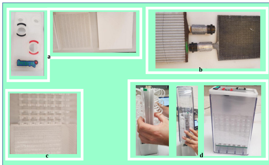
Figure 1: a) A new 3D-printed lid and separator frame with gas flow channels. b) Plates provided by Hoppecke and soldered to terminal blocks. c) An H&V separator was located within the new separator frame and H&V AGM and printed spring clips were used to provide pressure to the plates. d) Manufacture is straightforward – connect the terminals, assemble and slide the battery box on. Bubbles of hydrogen ( H_2 ) and oxygen ( O_2 ) appear at the output ports under electrolysis.
