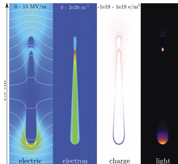
Figure 1: Positive streamer in air. The discharge growth results from the electric field enhancement at the head of the growing channel (source: [3]).
